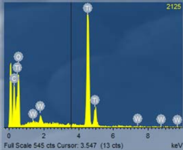
Suppl. 4. FE-SEM-EDS analysis from one W-rutile grain.
