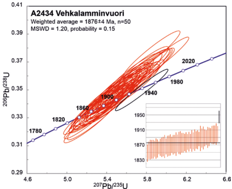
Fig. 7. U-Pb concordia diagram of the analysed quartz monzonite sample A2434. The spot of one older core is outlined in black. In inset ^{207}\text{Pb}/^{206}\text{Pb} ages of the spots. Data plotted at the 2\sigma level.
