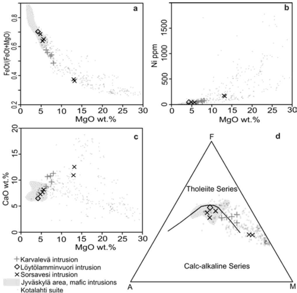
Fig. 8. Mafic samples from the Sorsakoski lithodeme plotted on a) MgO vs. FeO/(FeO+MgO) b) MgO vs. Ni c) MgO vs. CaO and d) Al 2 O 3 -FeO-MgO diagram (AFM, Irvine & Baragar 1971) diagrams. As reference data the mafic members of the Saarijärvi suite from Jyväskylä area (Virtanen & Heilimo 2018) and unmineralized Kotalahti suite samples with SiO 2 =40–55 wt.% from Leppävirta (Makkonen, unpublished data, n=333).
