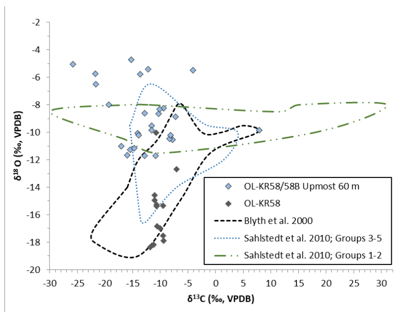
Figure 1. \delta^{13}\text{C} and \delta^{18}\text{O} values of calcite in the precipitate compared to reported values in fracture filling calcite at Olkiluoto. Groups 1-2 in Sahlstedt et al. (2010) represent latest calcite generations. Groups 3-5 represent older calcite generations.
