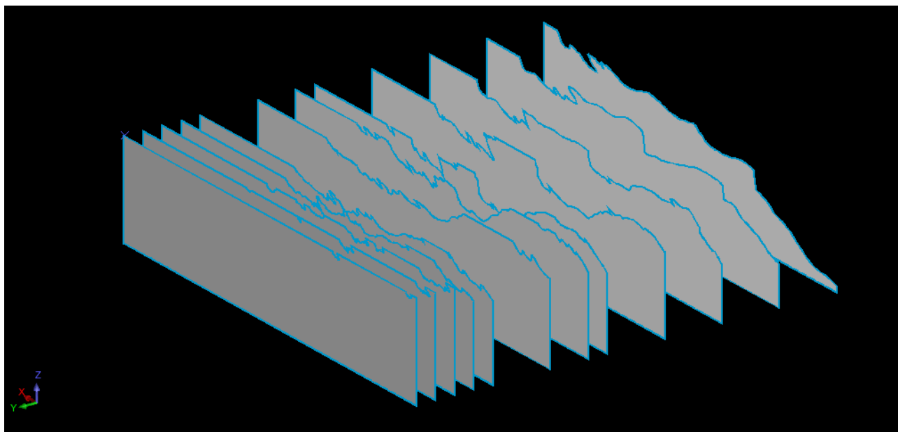
Figure C-2. Model profiles, view from NW. Profile spacings 5 – 15 km, depth extent 25 km.
