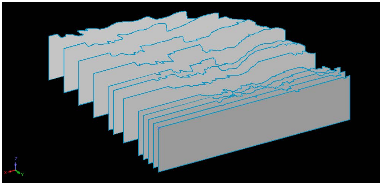
Figure C-1. Model profiles, view from NE. Profile spacings 5 – 15 km, depth extent 25 km.
