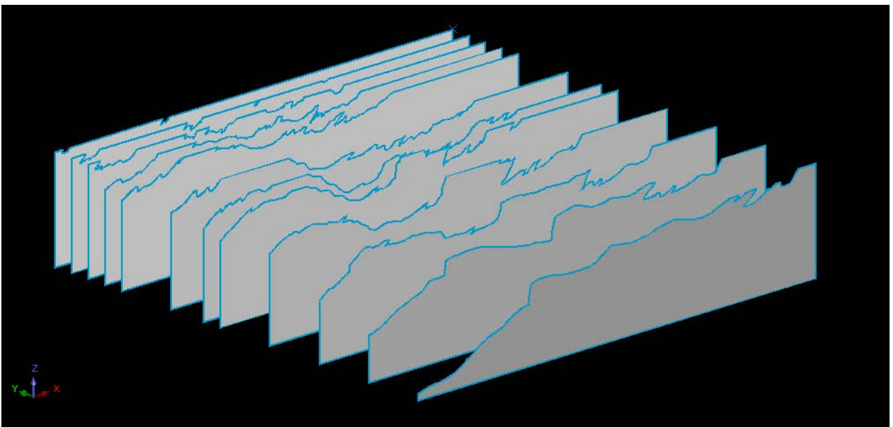
Figure C-4. Model profiles, view from SW. Profile spacings 5 – 15 km, depth extent 25 km.
