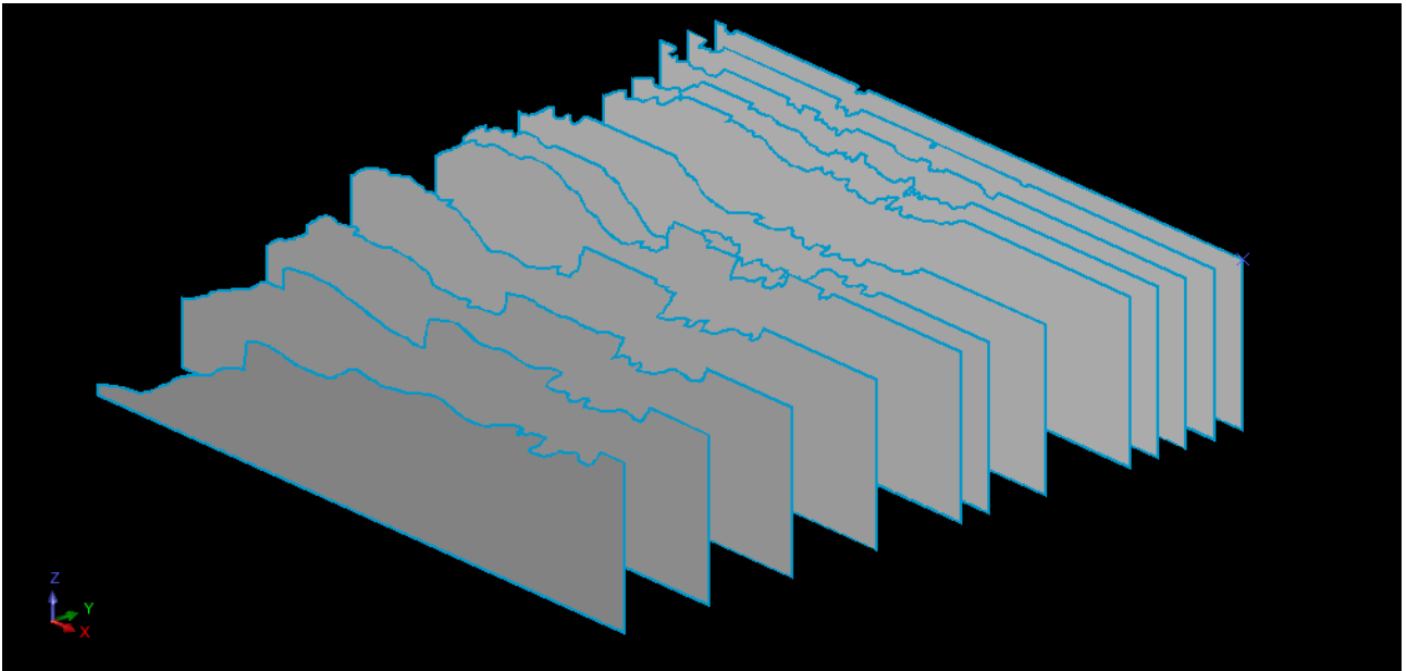
Figure C-3. Model profiles, view from SE. Profile spacings 5 – 15 km, depth extent 25 km.
