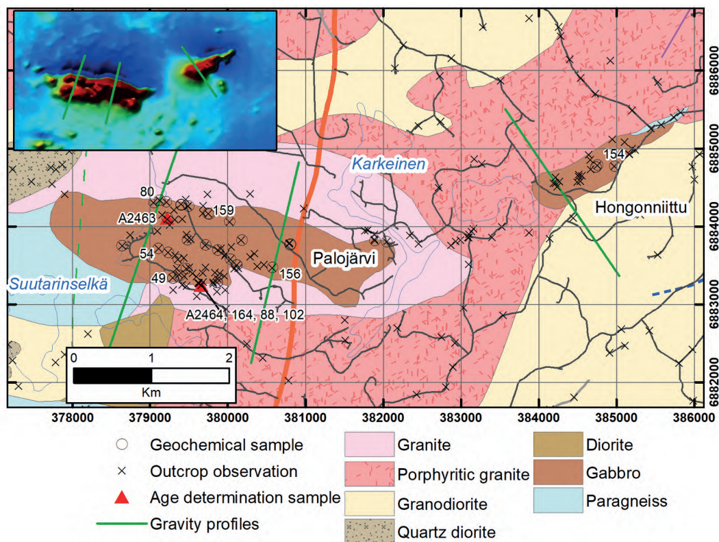
Figure 3. Geological map of the Palojärvi and Hongonniittu intrusions displaying sample and observation sites. SIKA-2017- has been omitted from the site numbers for brevity. Map modified from Bedrock map of Finland - DigiKP. In inset aeromagnetic map of the same area, red indicates high and blue low values. Green lines indicate the gravity measurement lines
