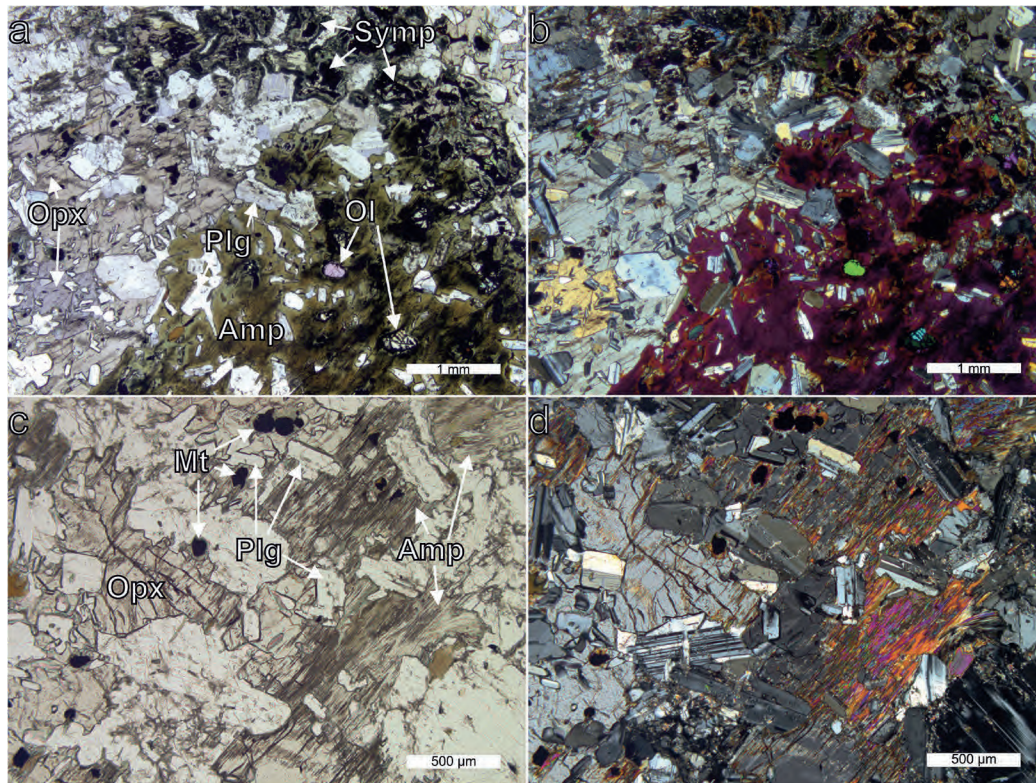
Figure 8. Optical microscope pictures of olivine-hornblende-norite (sample SIKA-2017-80.1, Palojärvi). Oikocrystic amphibole (amp) and orthopyroxene (opx) enclosing cumulus plagioclase (plg) and olivine (ol). Olivine is often oxidized to magnetite. Notice the symplectites (Symp; a, b), where olivine is surrounded by orthopyroxene and a reaction rim against plagioclase. c, d) Secondary acicular amphibole with orange-red interference colors is replacing orthopyroxene. a) and c) are in plane-polarized light, b) and d) in cross-polarized light.
